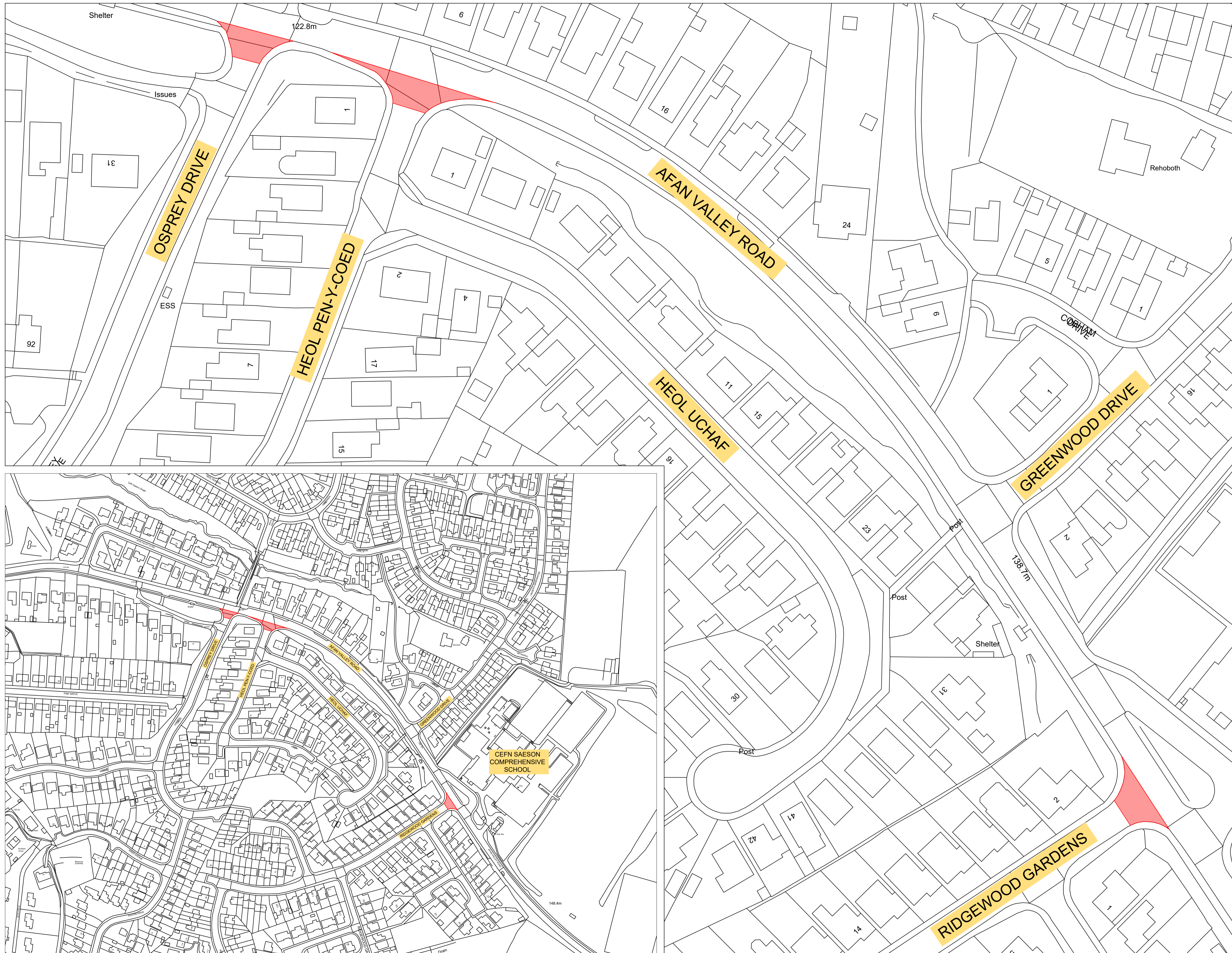
LOCATION PLAN SCALE 1:2000
